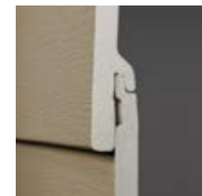
Celect's unique gravity lock design keeps courses locked tight to maintain structural integrity.
