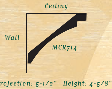
MCR714 Ceiling Step
