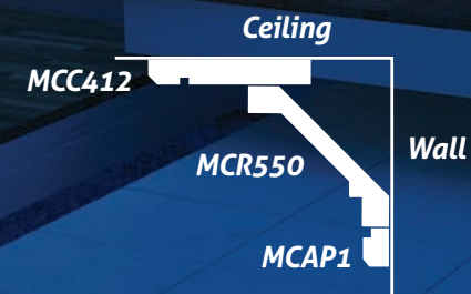
MCR550 Step on Wall, MCAP1, MCC412
