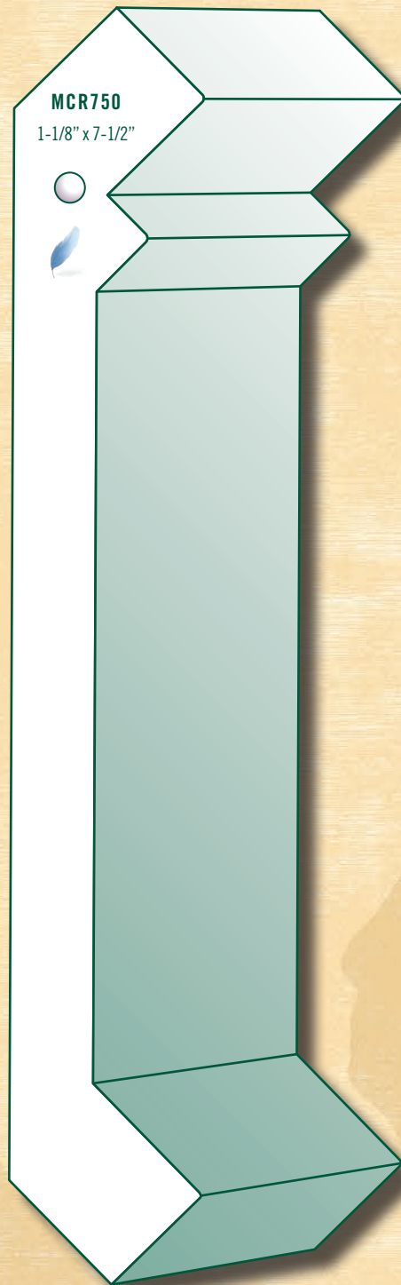
MCR750 Step on Wall, MCAP34
