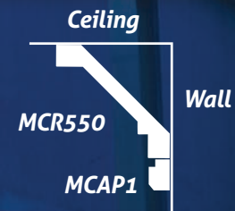
MCR550 Step on Wall, MCAP1
