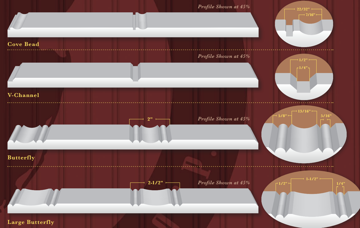
Cove Bead (3-1/2" On Center), Cap Combination: 1x4, SC214, FS312
