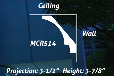
MCR514 Wall Step
