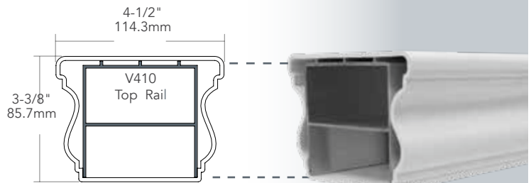
Top Rail
