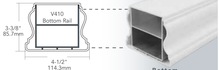
Bottom Rail
