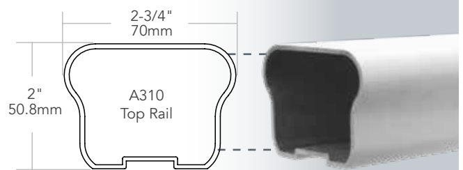
Top Rail
