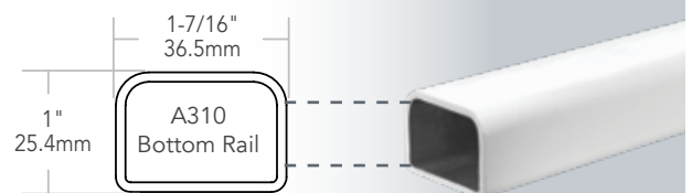
Bottom Rail
