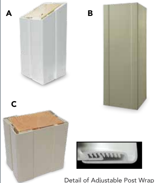
Detail of Adjustable Post Wrap Ratcheting System Adjustable in 0.125" Increments
