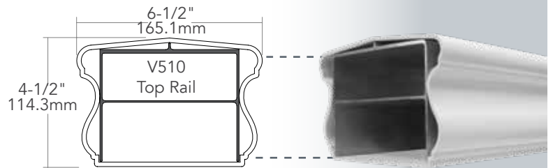
Top Rail
