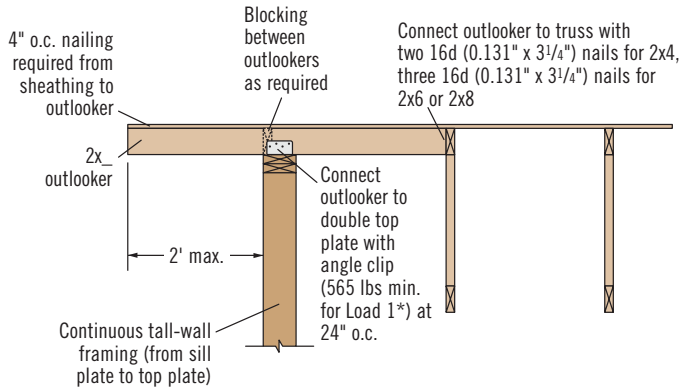
WB2 * Load 1 value from Lateral Connections—Angle Clips table below.
