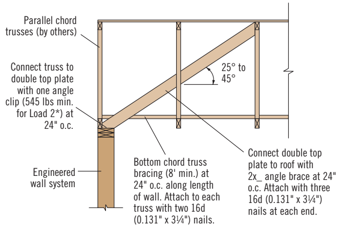
WB3 * Load 2 value from Lateral Connections—Angle Clips table below.
